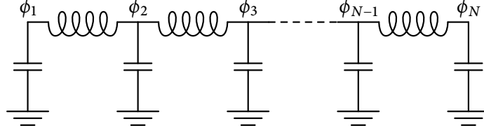
Figure 2.2: The transmission line. The figure shows a transmission line with open-circuit boundary conditions, represented as the continuum limit of a chain of LC oscillators.
